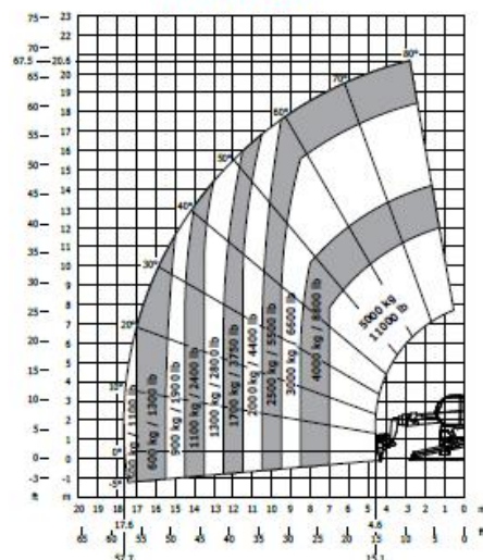
Rotation on lowered stabilizers with 1500 kg jib
