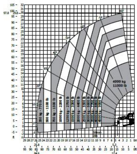
Rotation on lowered stabilizers with forks
