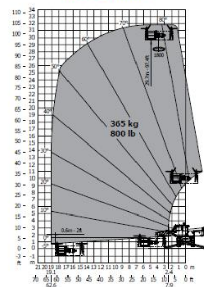
Rotation on lowered stabilizers with 365 kg platform
