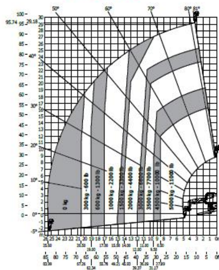
Rotation on lowered stabilizers with 1500 kg jib
